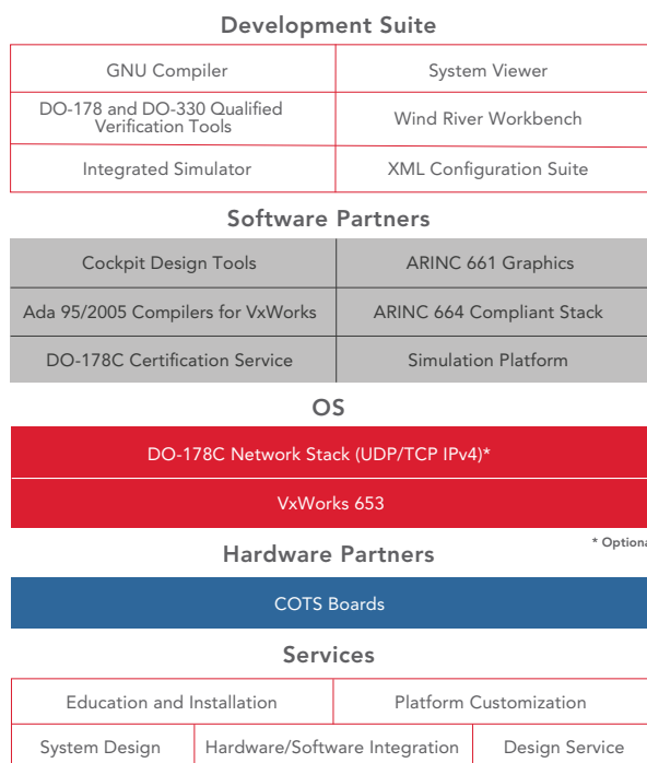
Figure 1. VxWorks 653 Multi-core Edition
